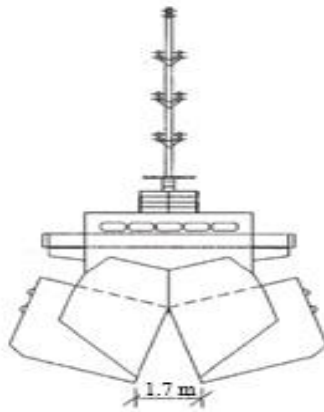
Section looking aft hopper open
