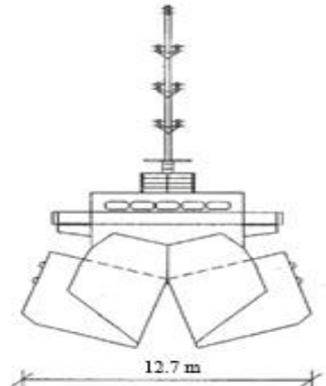
Section looking aft hopper open
